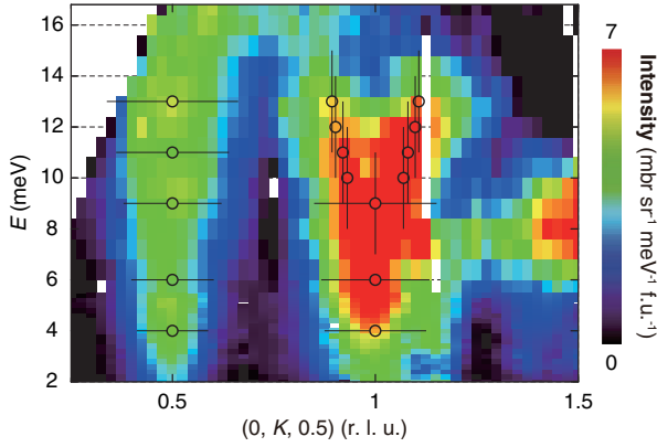
FIG. 2. Dispersions of the stripe ( K \sim 0.5 ) and the ferromagnetic spin fluctuations ( K \sim 1 ) in \text{YFe}_2\text{Ge}_2 at 4 K. The low-energy ( E < 5.6 meV) and the high-energy ( 5.6 meV < E < 16.8 meV) parts were measured on AMATERAS with incident neutron energies of 15 and 42 meV, respectively. The |\mathbf{Q}| -dependent background subtraction and intensities normalization were performed in the same way as in Fig. 1. The open circles represent for the peak positions determined from the Gaussian fitting of the constant-energy scans. The horizontal bars show the full width at half maximum (FWHM) of the peaks, while the vertical bars indicate the range of integrated energies.
